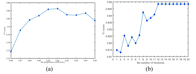
Fig. 10. Influence of the (a) coefficient \epsilon on discrimination performance and (b) Number of iterations on discrimination performance when \epsilon = 0.91 .
