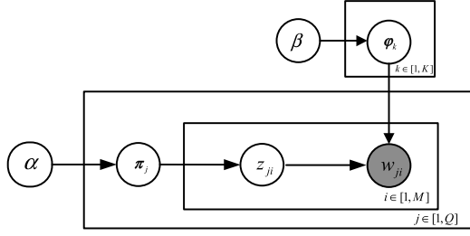
Fig. 4. Generated model of LDA.
