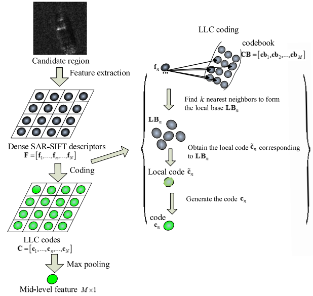
Fig. 2. Procedure of mid-level feature generation.
