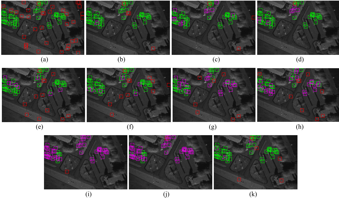
Fig. 13. Annotation diagram of discrimination results on the images shown in Fig. 5(d) via different discrimination methods, where the green rectangles represent correctly discriminated vehicle targets, the red rectangles represent false alarms, and the magenta rectangles represent missed targets. (a) Reference image. (b) The proposed method. (c) Linear SVM 1. (d) Linear SVM 2. (e) QDD1. (f) QDD2. (g) QPD1. (h) QPD2. (i) Linear SVDD 1. (j) Linear SVDD 2. (k) WSL in [32].
