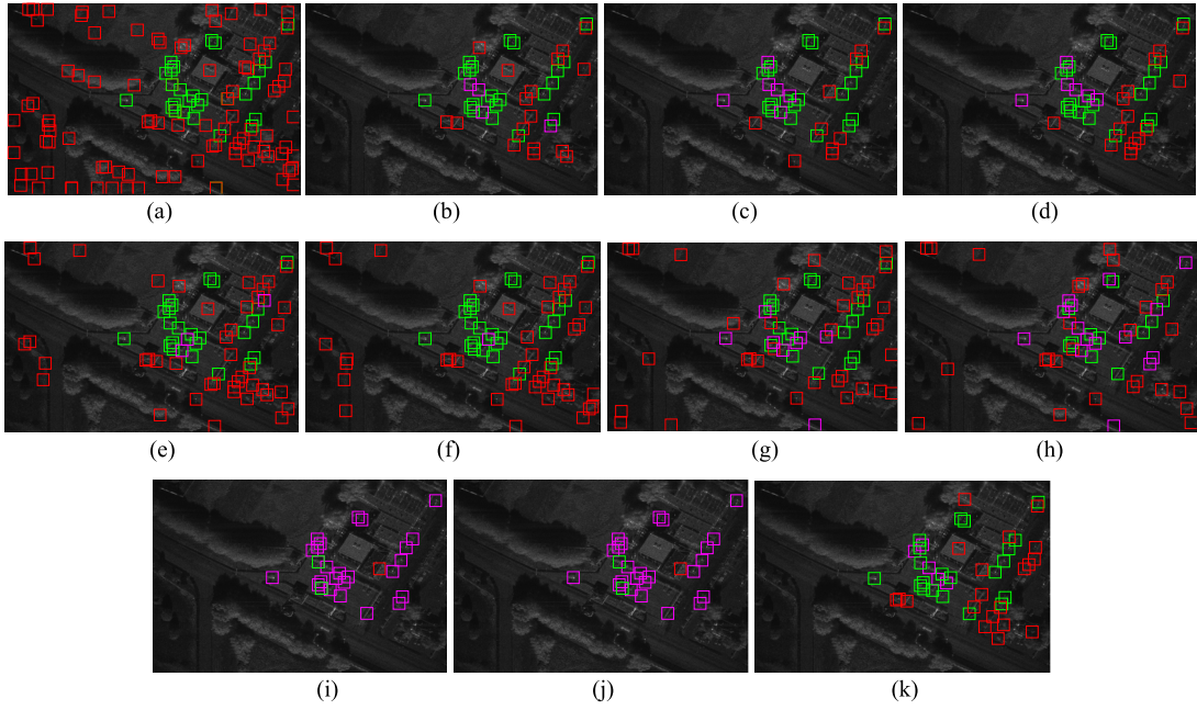
Fig. 12. Annotation diagram of discrimination results on the images shown in Fig. 5(c) via different discrimination methods, where the green rectangles represent correctly discriminated vehicle targets, the red rectangles represent false alarms and the magenta rectangles represent missed targets. (a) Reference image. (b) The proposed method. (c) Linear SVM 1. (d) Linear SVM 2. (e) QDD1. (f) QDD2. (g) QPD1. (h) QPD2. (i) Linear SVDD 1. (j) Linear SVDD 2. (k) WSL in [32].
